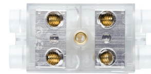
SFBW22C UNDERSIDE
